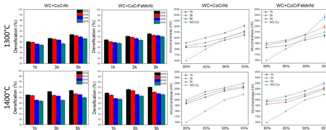
Figure 3. Values of densification and microhardness obtained from the WC-CoCrNi and WC-CoCrFeMnNi systems sintered at 1300 and 1400°C.
